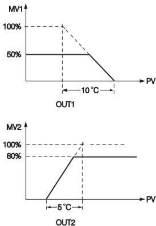
Figure 4-52. Power Limit Function
