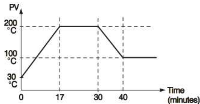
Figure 4-48.Ramp Function
