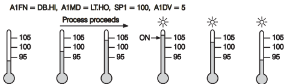
Figure 4-47.Latching/Holding Deviation Band Alarm
