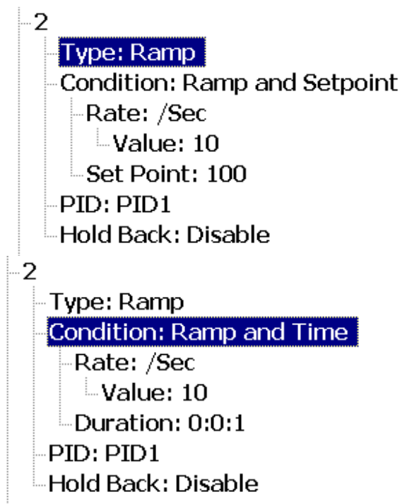
Figure 4-60.Ramp Segment
