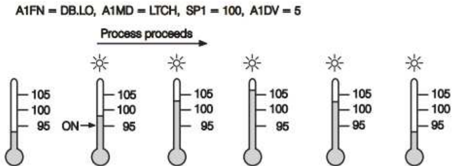
Figure 4-45.Latching Deviation Band Alarm
