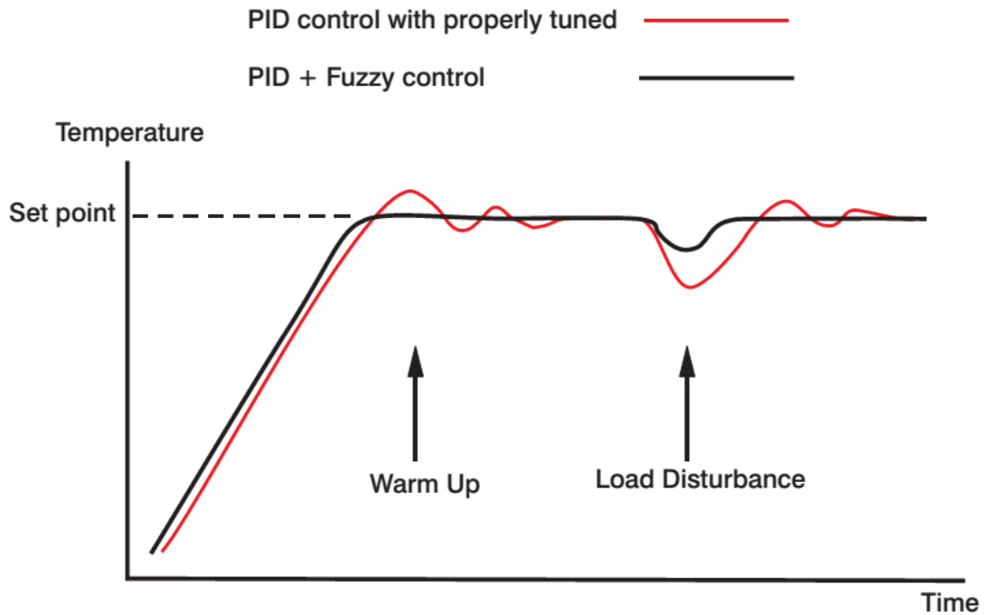
Figure 1-2. PID System Stability with and without Fuzzy
