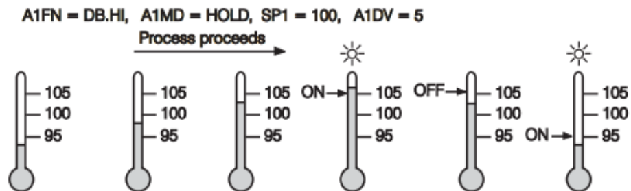
Figure 4-46.Holding Deviation Band Alarm
