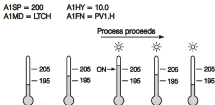
Figure 4-36. Normal Process Alarm
