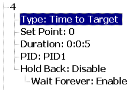
Figure 4-67. Time To Target Segment
