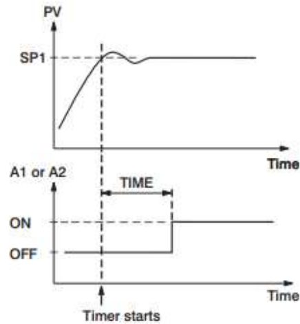
Figure 4-35.Dwell Timer
