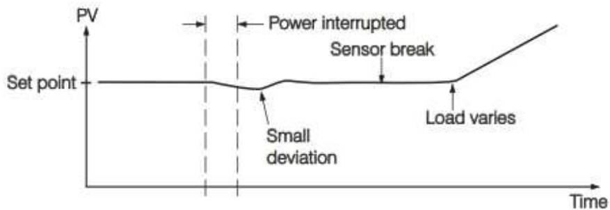
Figure 4-32. With Bumpless Transfer
