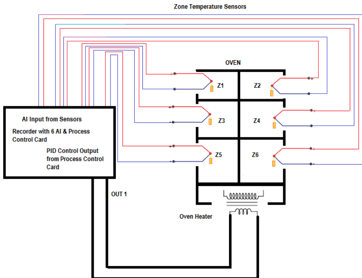
Figure 5-1. Oven Control with Zone Temperature Recording
