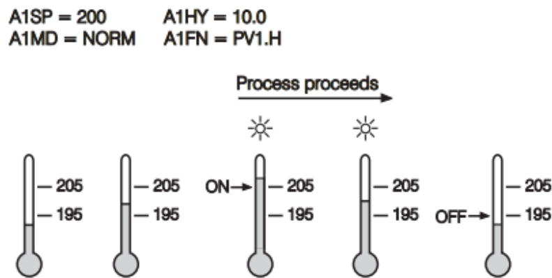
Figure 4-36. Normal Process Alarm
