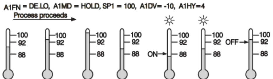
Figure 4-42.Holding Deviation Alarm
