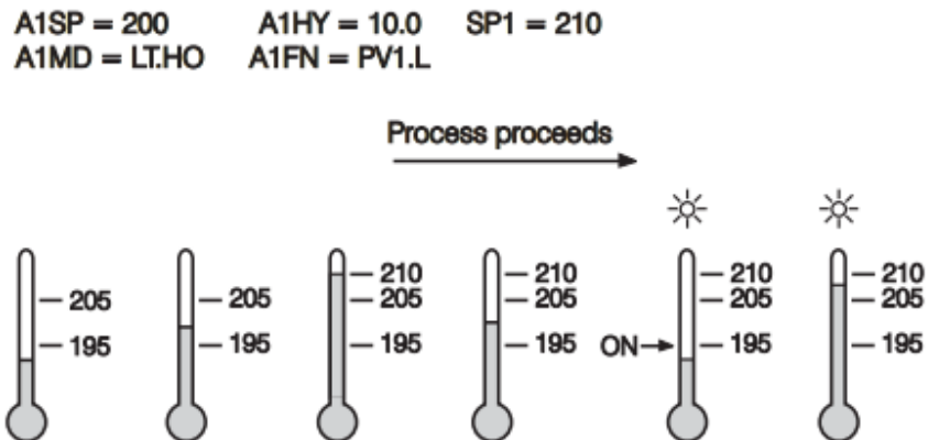
Figure 4-39.Latching / Holding Process Alarm
