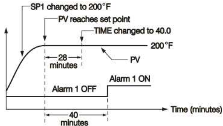
Figure 4-49.Dwell Timer
