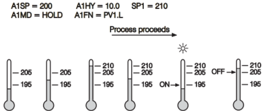
Figure 4-38.Holding Process Alarm
