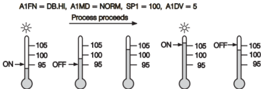
Figure 4-44. Normal Deviation Band Alarm
