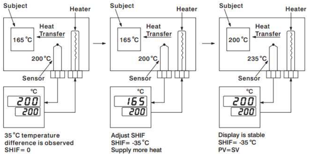
Figure 4-33.PV1 SHIFT Application
