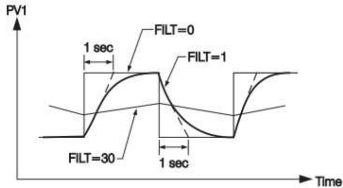
Figure 4-53. Filter Characteristics
