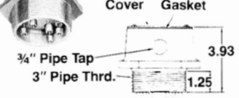
TYPE E-4 TO E-7
