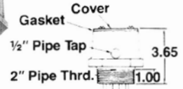
TYPE E-2 & E-3
