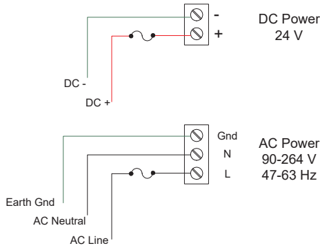
Figure 1. Power Connections
