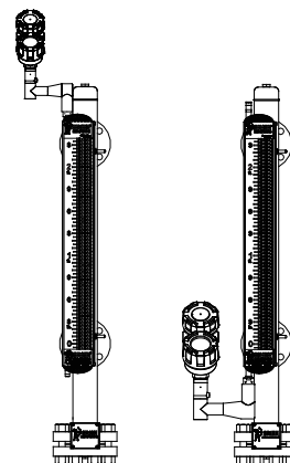
Top/Bottom Mount Offset Configuration
