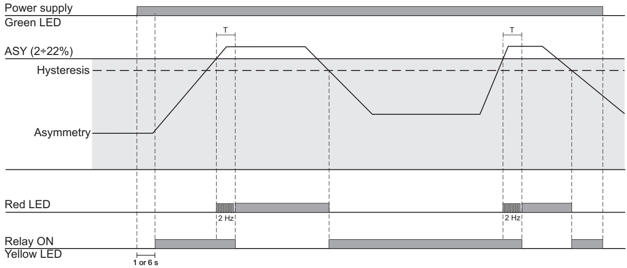
Fig. 6 Asymmetry monitoring
