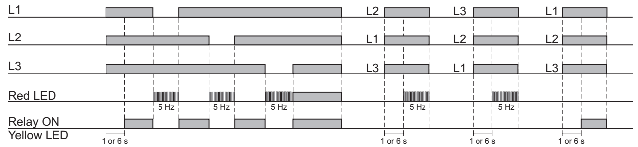
Fig. 7 Phase sequence and phase loss monitoring
