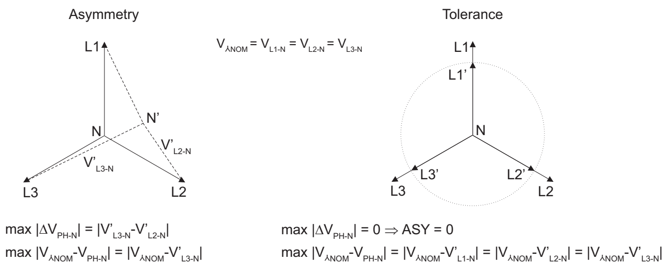
Fig. 2 Phase-neutral monitoring
